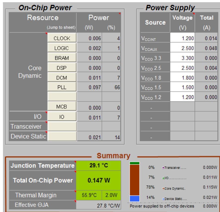
Figure 8: Updated Power and Thermal Distribution in XPE for Spartan-6 FPGA
