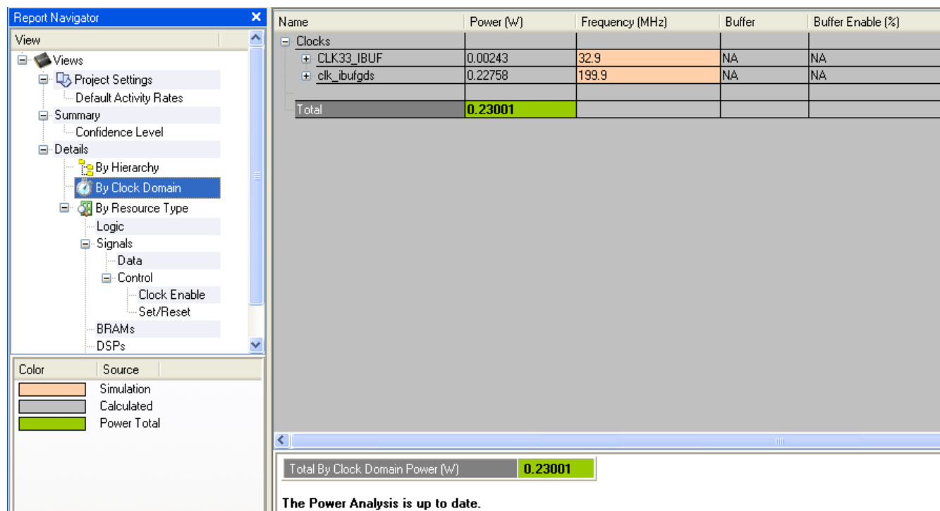
Figure 12: By Clock Domain View - XPower Analyzer (XPA)
