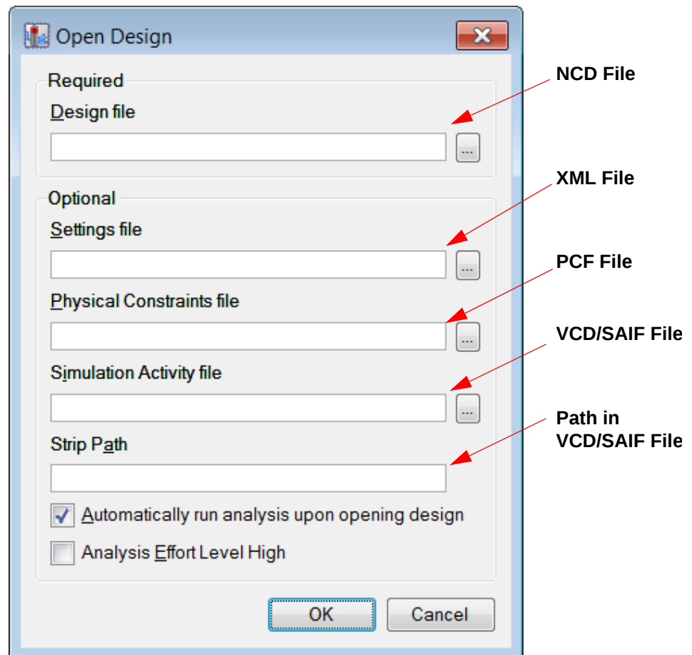
Figure 9: Open Design Dialog Box (XPA)
