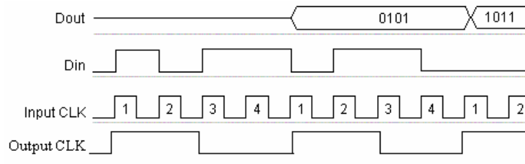
Serial to Parallel
