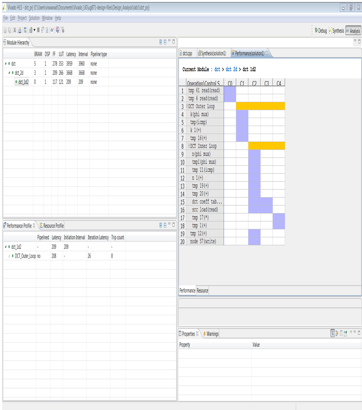
Figure 6-12: DCT_1D Performance View
