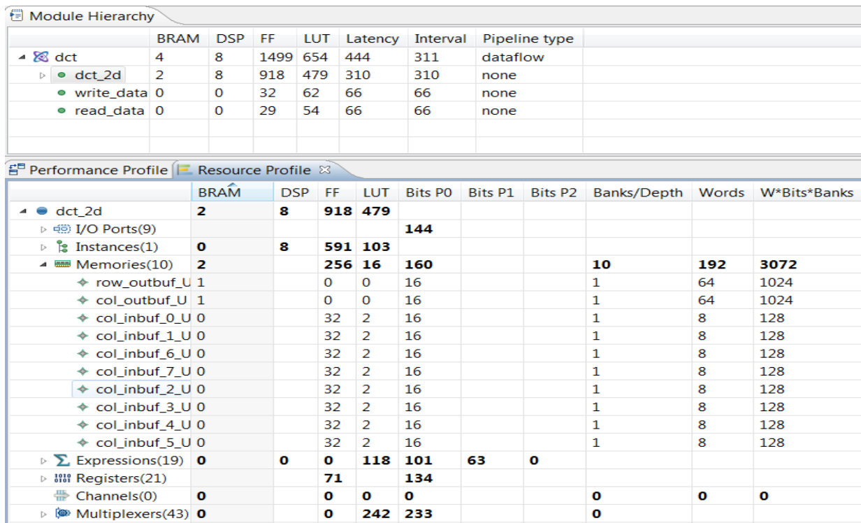
Figure 6-32: DCT Resource Profile
