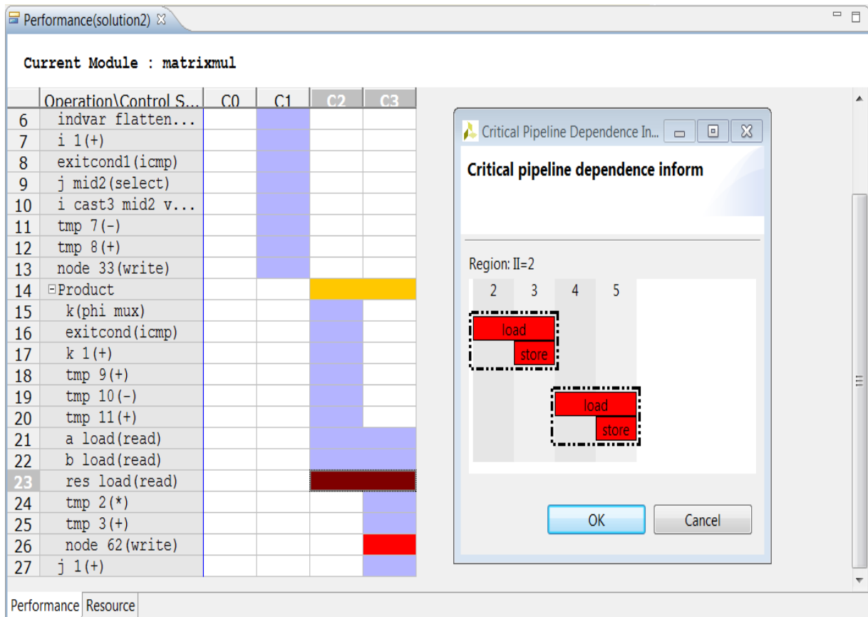
Figure 7-9: Carried Dependency Analysis
