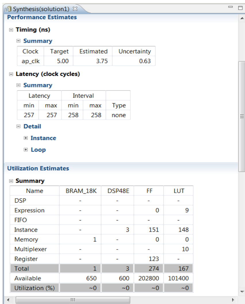
Figure 5-6: Synthesis Report for Floating Point Design
