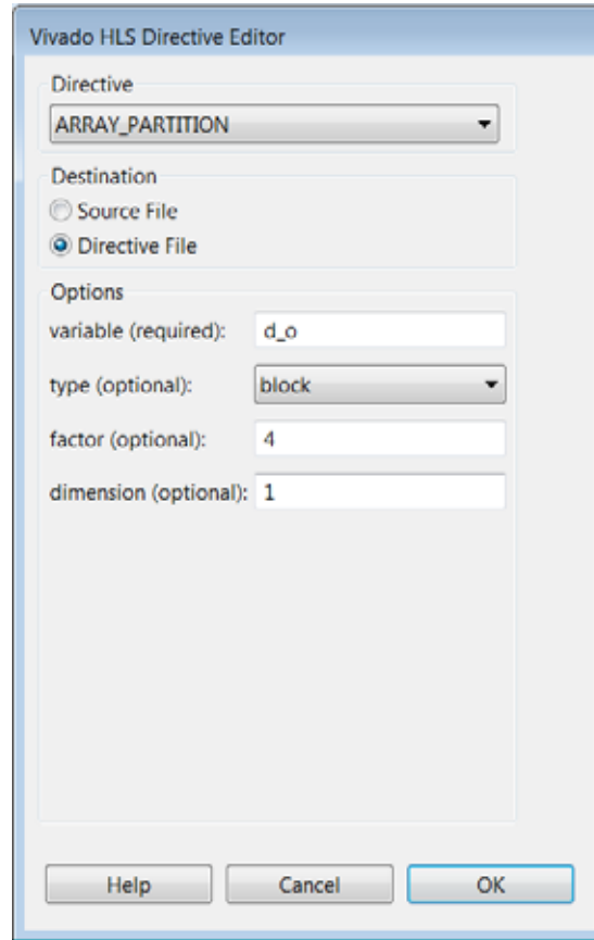
Figure 4-22: Directives Editor for Partitioning Array d_o
