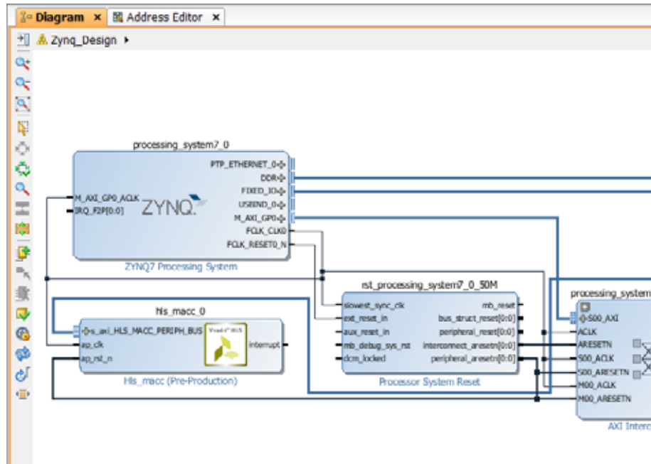
Figure 10-18: Design with AXI4 Interconnect
