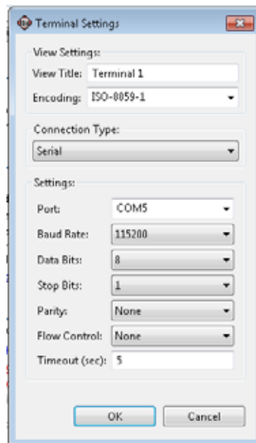
Figure 10-24: Terminal Settings
