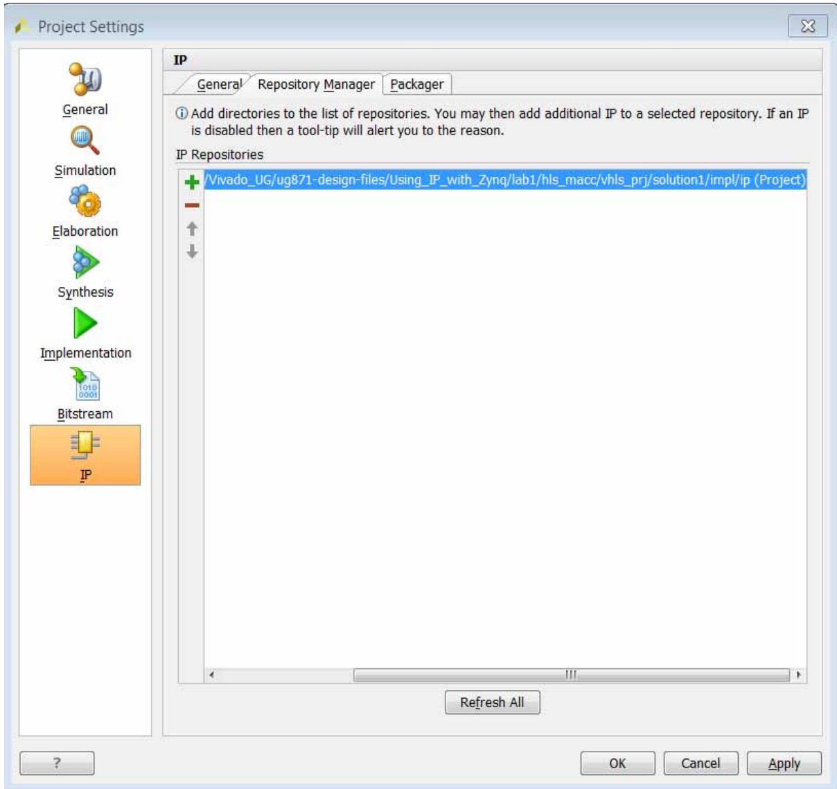
Figure 10-9: IP Repository
