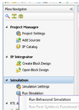
Figure 9-28: Execute Simulation
