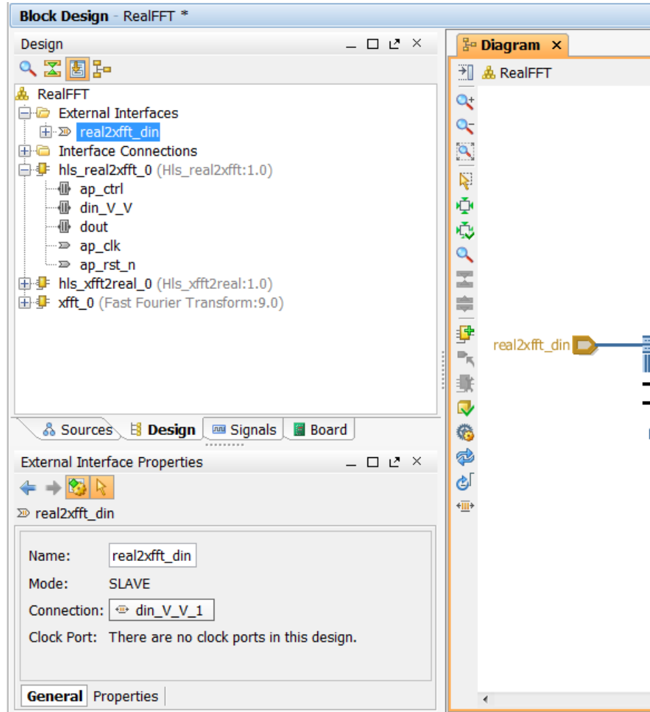
Figure 9-20: Port Naming
