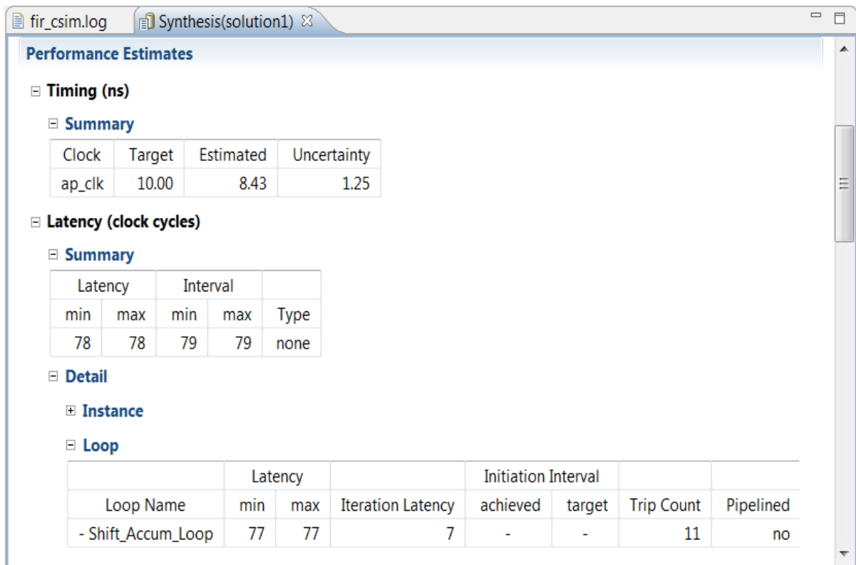
Figure 2-11: Performance Estimates
