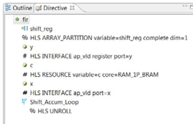
Figure 2-28: Solution3 Directives
