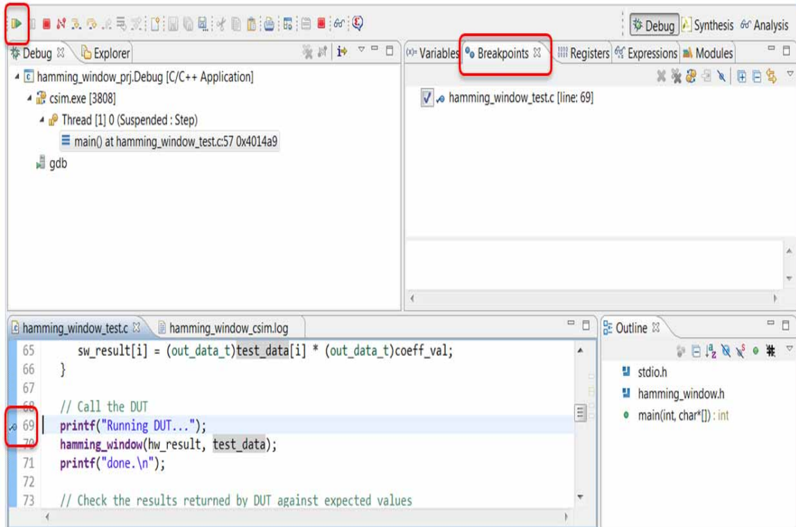
Figure 3-11: Using Breakpoints
