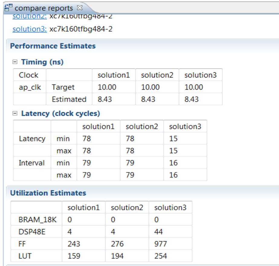
Figure 2-30: Comparison of Lab3 Solutions
