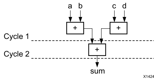
Figure 1-70: Adder Tree After Balancing
