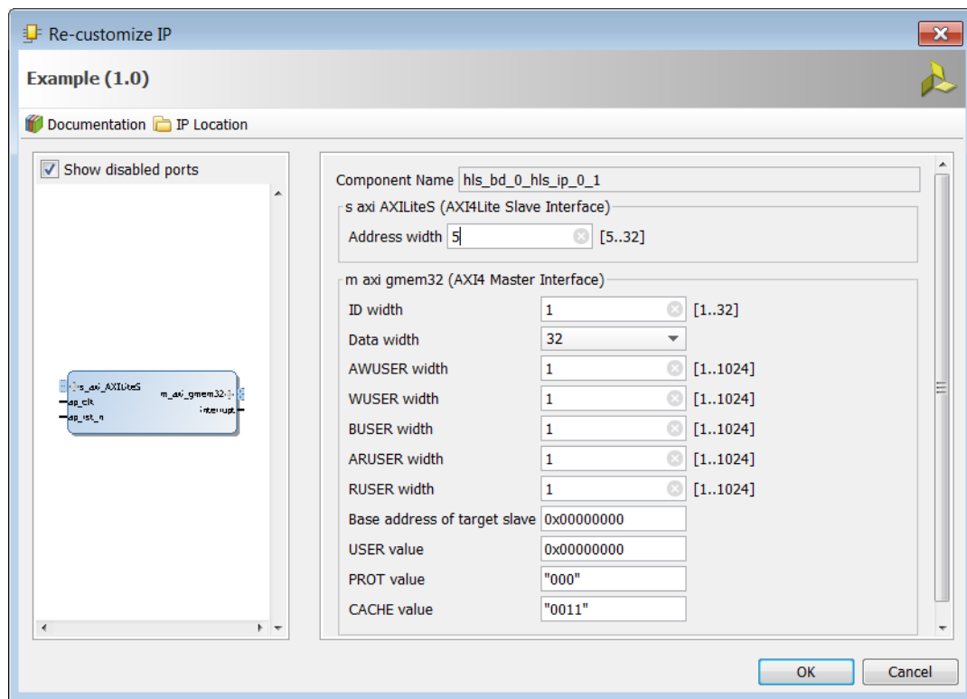
Figure 1-46: Customizing AXI4 Master Interfaces in IP Integrator
