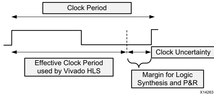
Figure 1-47: Clock Period and Margin
