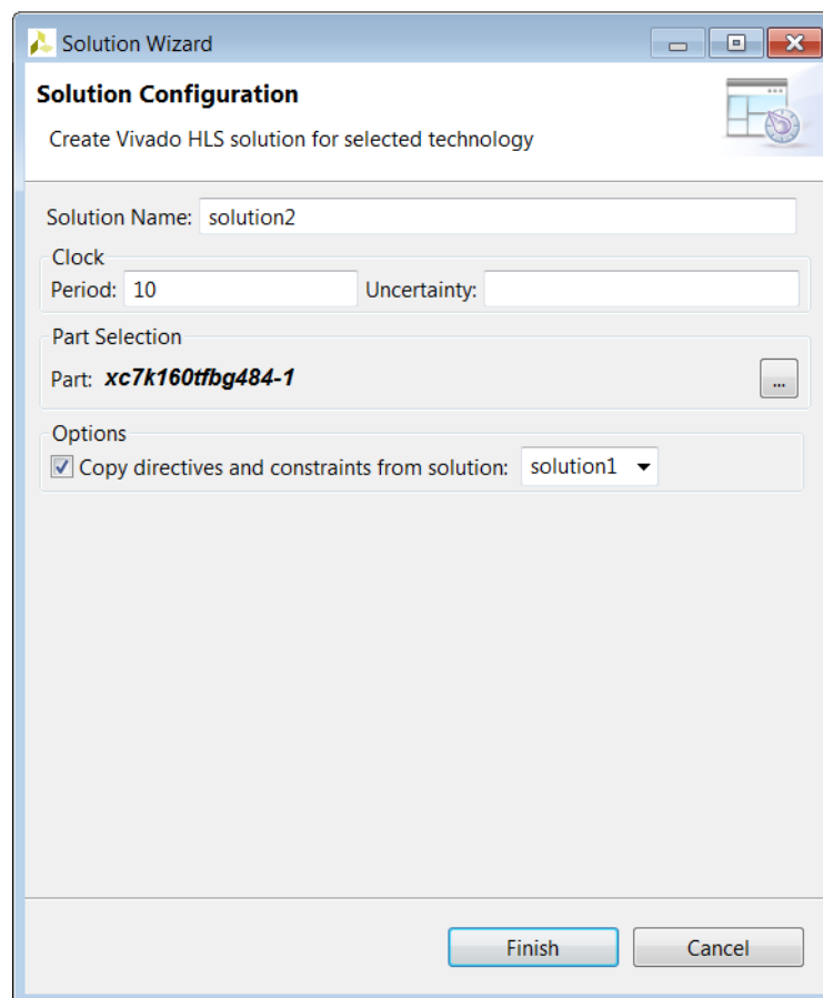
Figure 1-26: New Solution Wizard
