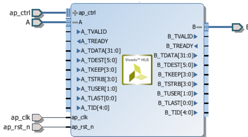
Figure 1-42: Pcore: AXI4-Stream Interfaces
