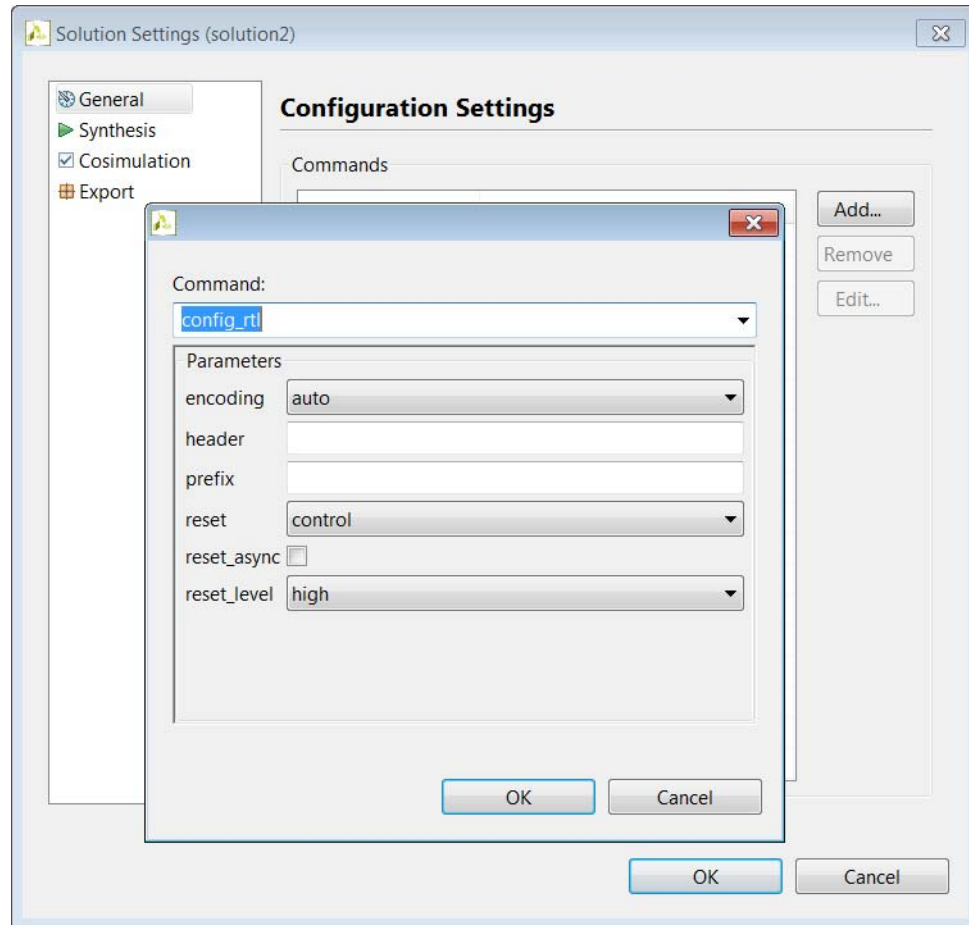
Figure 1-48: RTL Configurations
