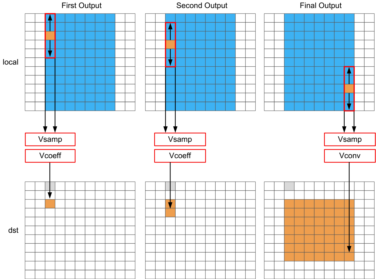
Figure 3-3: Vertical Convolution
