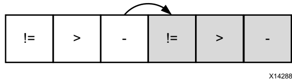
Figure 1-57: Scalar Dependency
