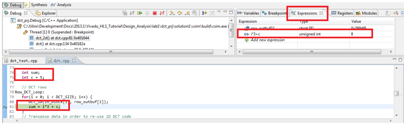
Figure 4-2: Monitoring Expressions
