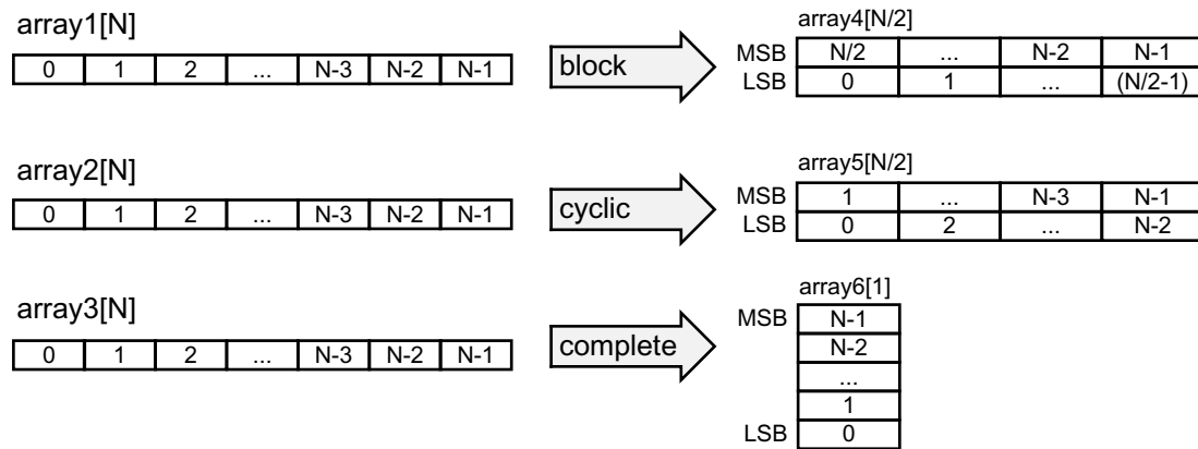
Figure 1-68: Array Reshaping
