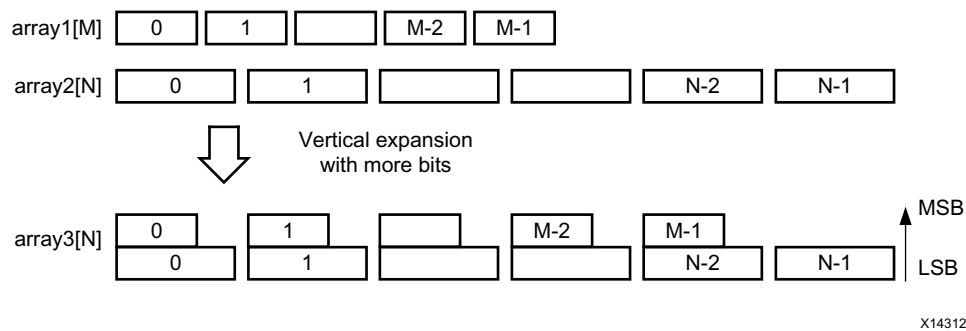
Figure 1-66: Vertical Mapping
