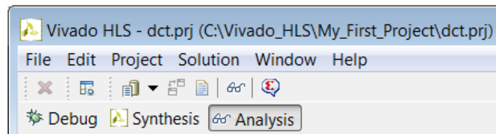
Figure 1-22: Analysis Perspective
