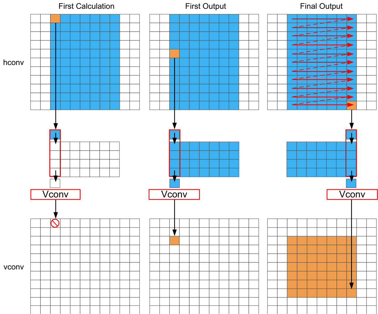
Figure 3-7: Streaming Vertical Convolution
