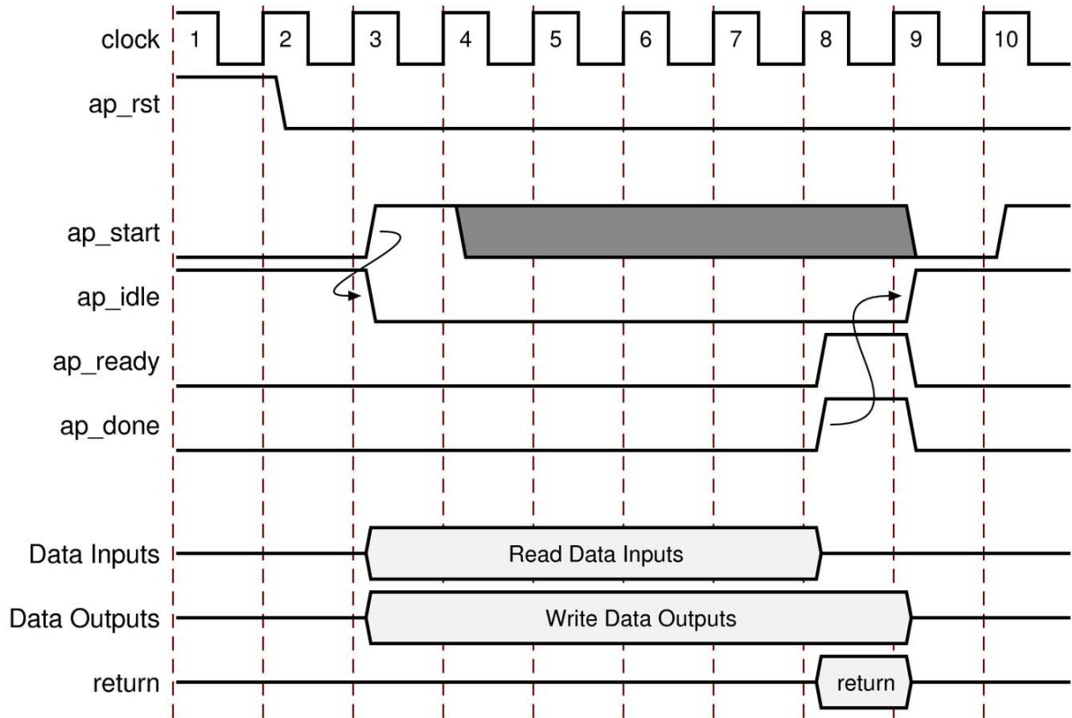
Figure 4-6: Behavior of ap_ctrl_hs Interface
