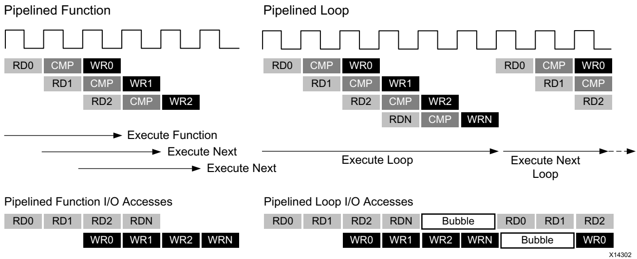
Figure 1-51: Function and Loop Pipelining Behavior
