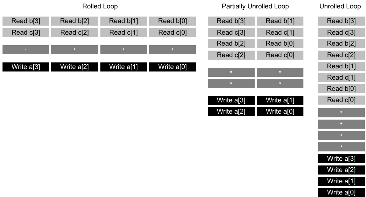
Figure 1-58: Loop Unrolling Details
