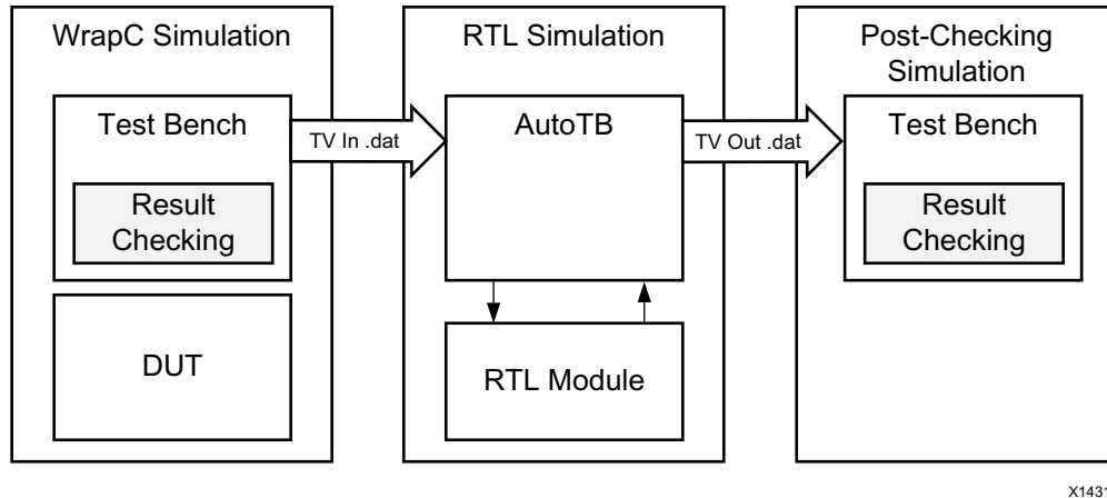
Figure 1-71: RTL Verification Flow
