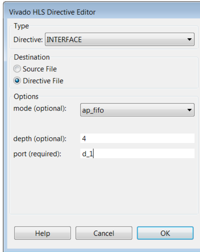
Figure 3-1: Vivado HLS Directive Editor with Depth Option
