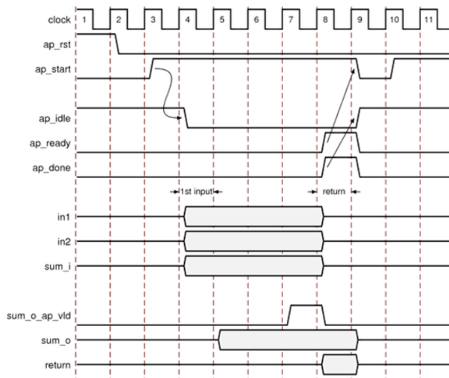
Figure 1-37: RTL Port Timing with Default Synthesis
