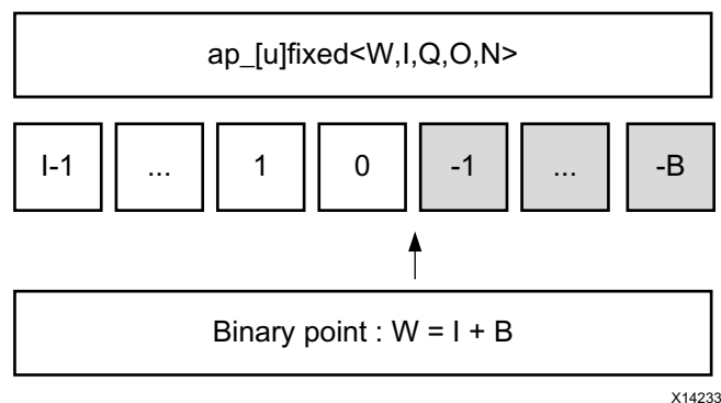
Figure 2-3: Arbitrary Precision Fixed-Point Types
