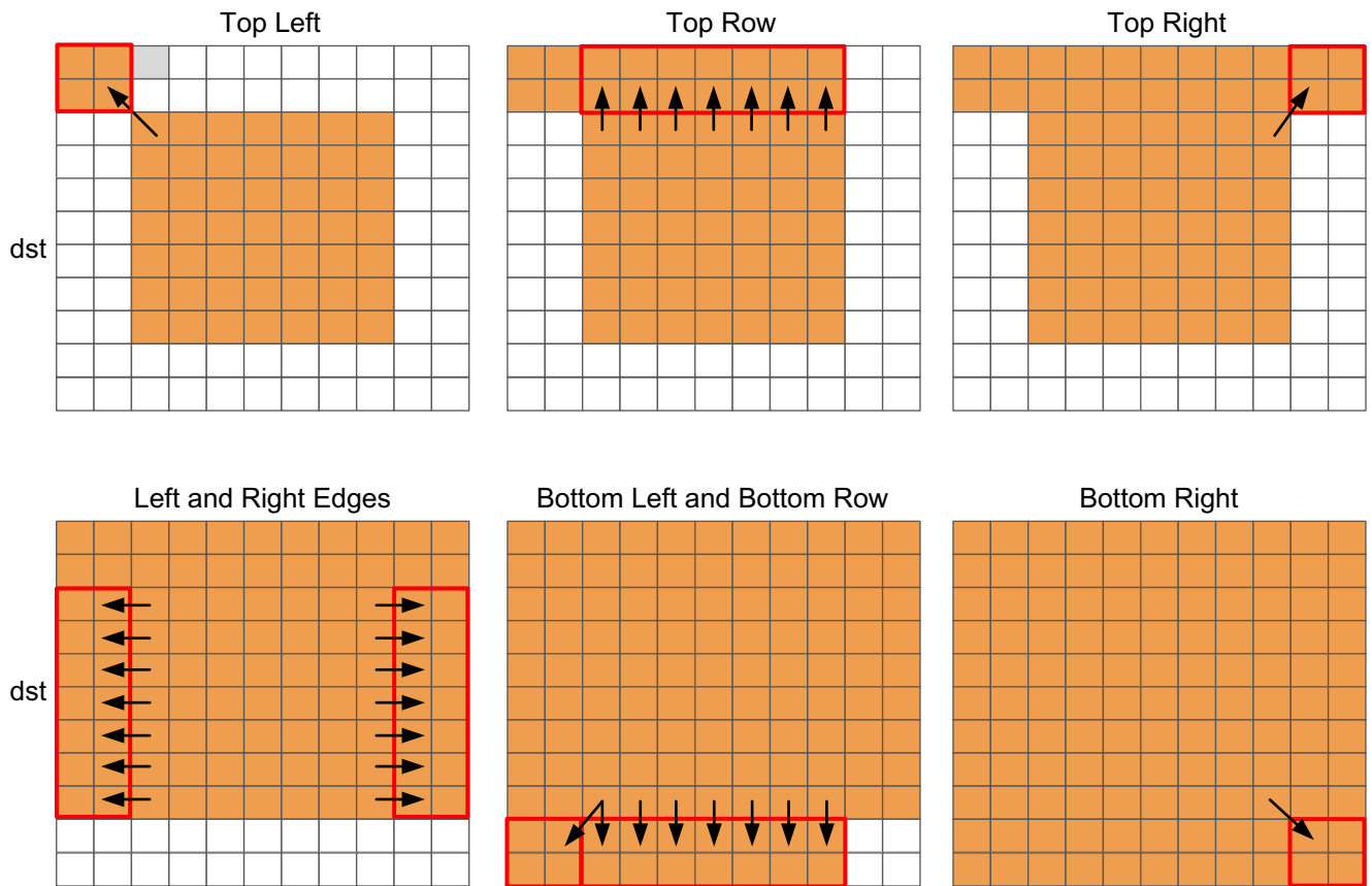
Figure 3-4: Convolution Border Samples
