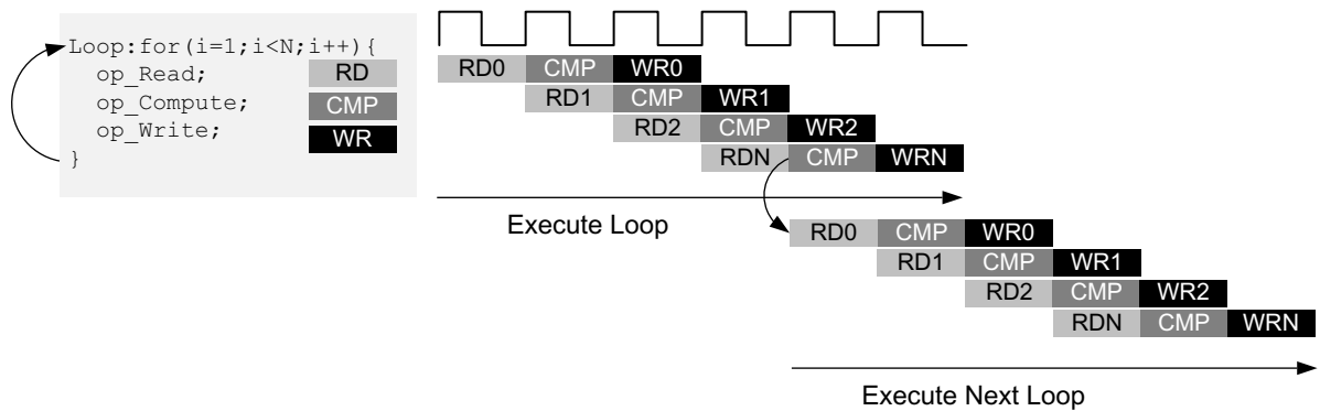
Figure 1-52: Loop Pipelining with Rewind Option
