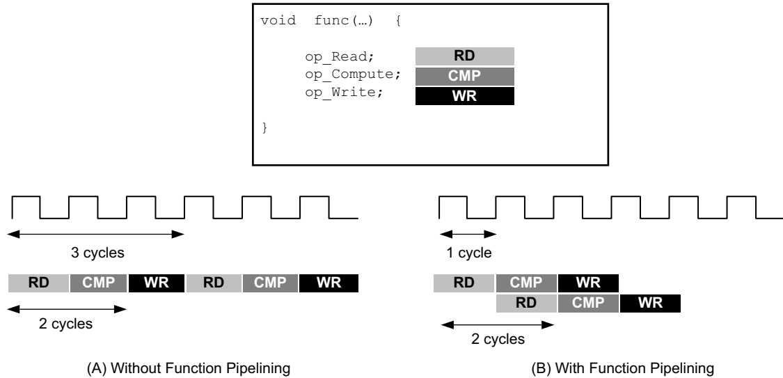
Figure 1-49: Function Pipelining Behavior
