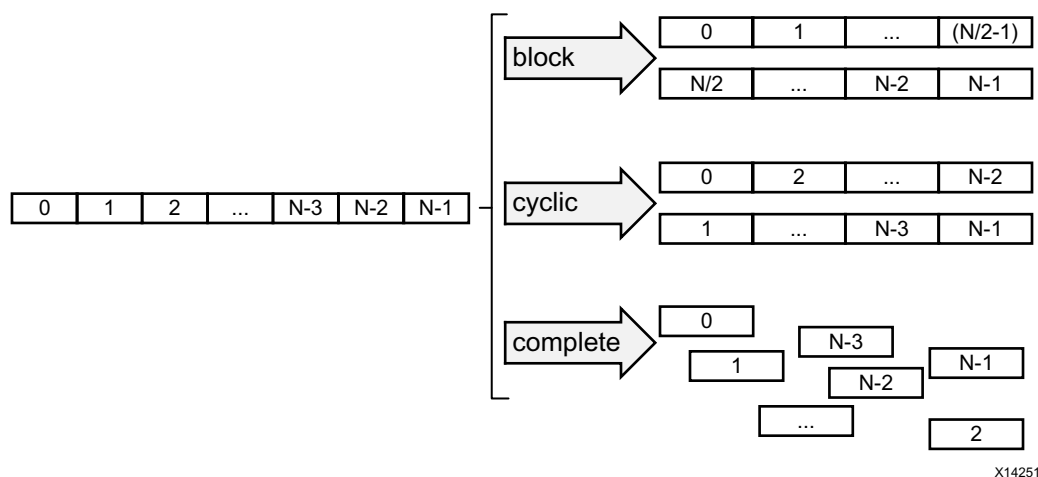
Figure 1-54: Array Partitioning
