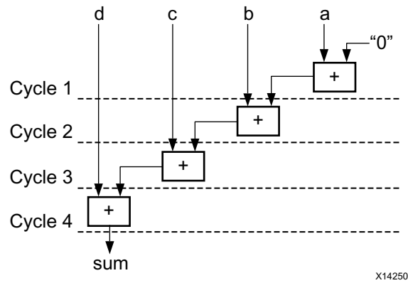
Figure 1-69: Adder Tree
