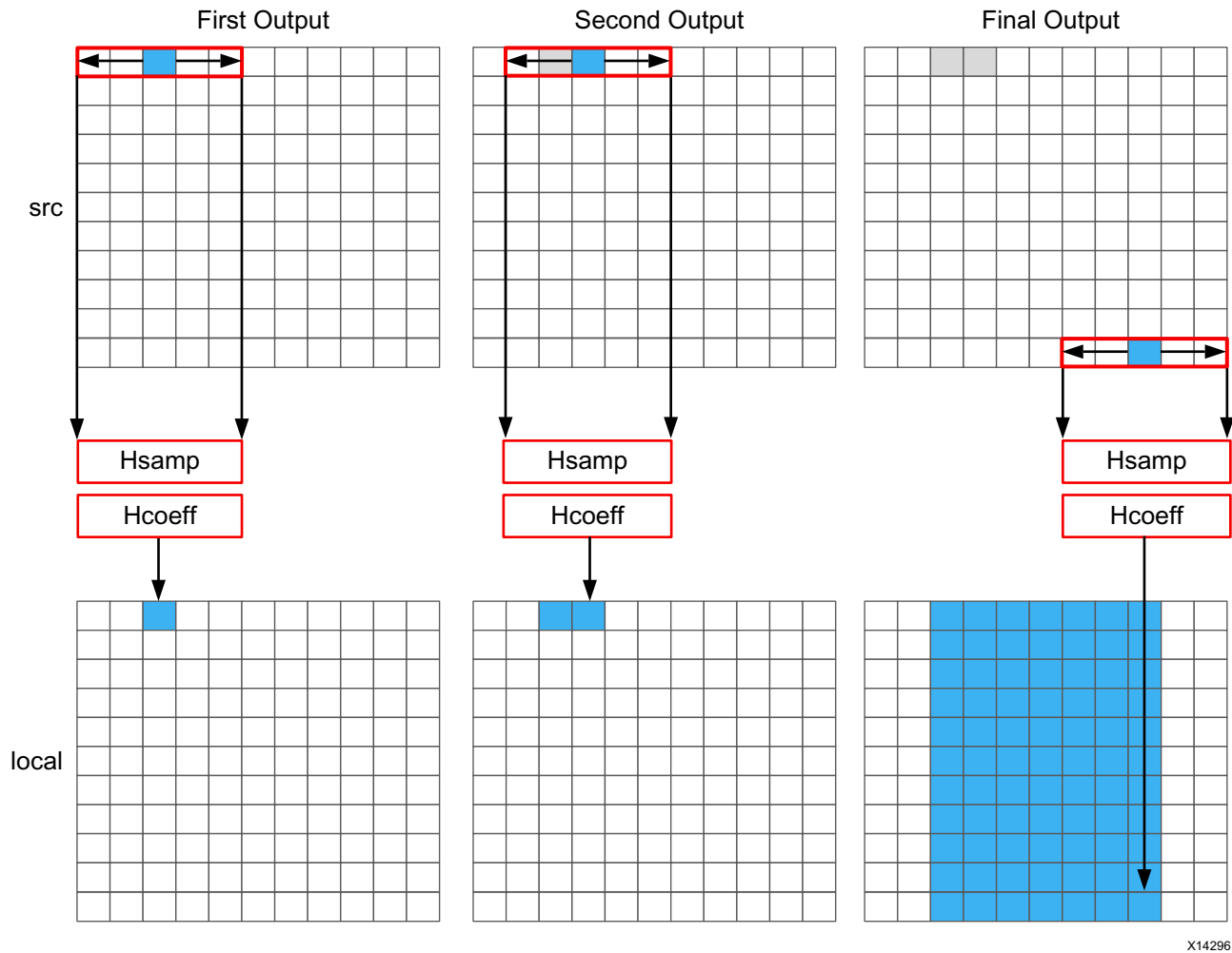
Figure 3-2: Horizontal Convolution
