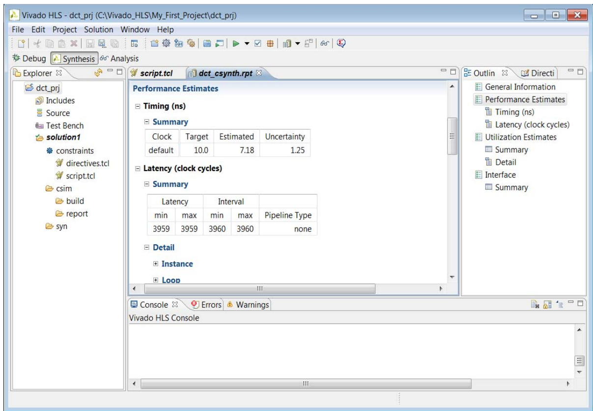
Figure 1-19: Synthesis Report
