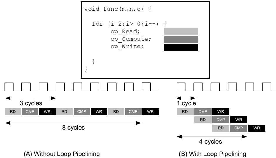
Figure 1-50: Loop Pipelining
