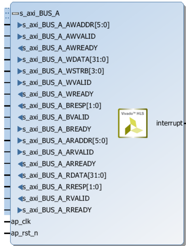
Figure 1-43: AXI4-Lite Slave Interfaces with Grouped RTL Ports
