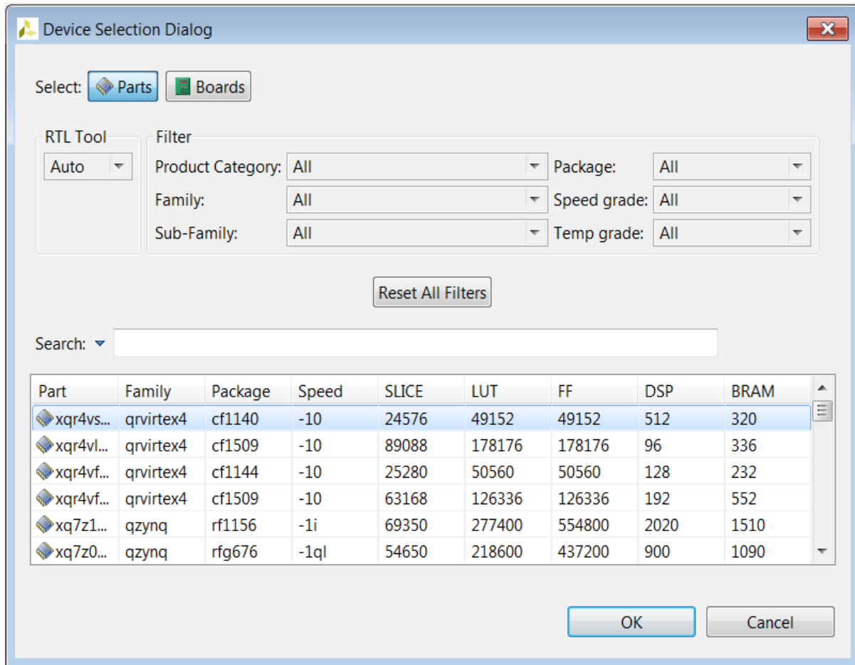
Figure 1-13: Part Selection
