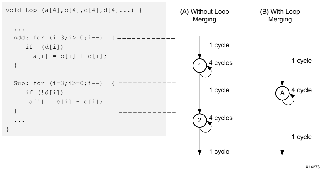
Figure 1-62: Loop Directives
