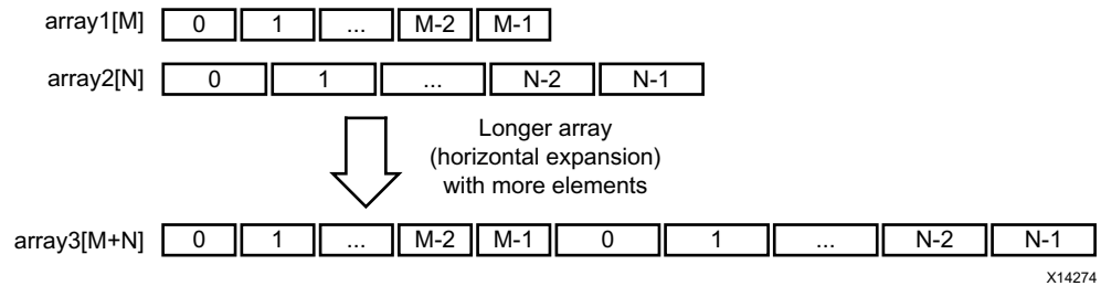
Figure 1-63: Horizontal Mapping
