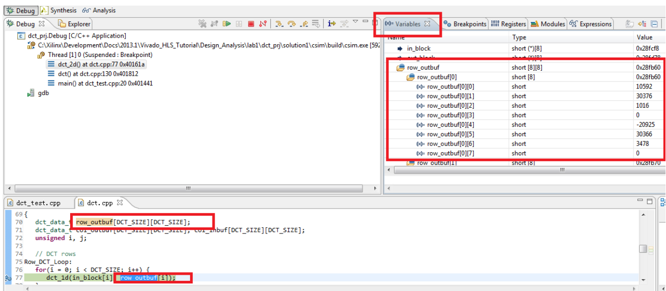
Figure 4-1: Monitoring Variables
