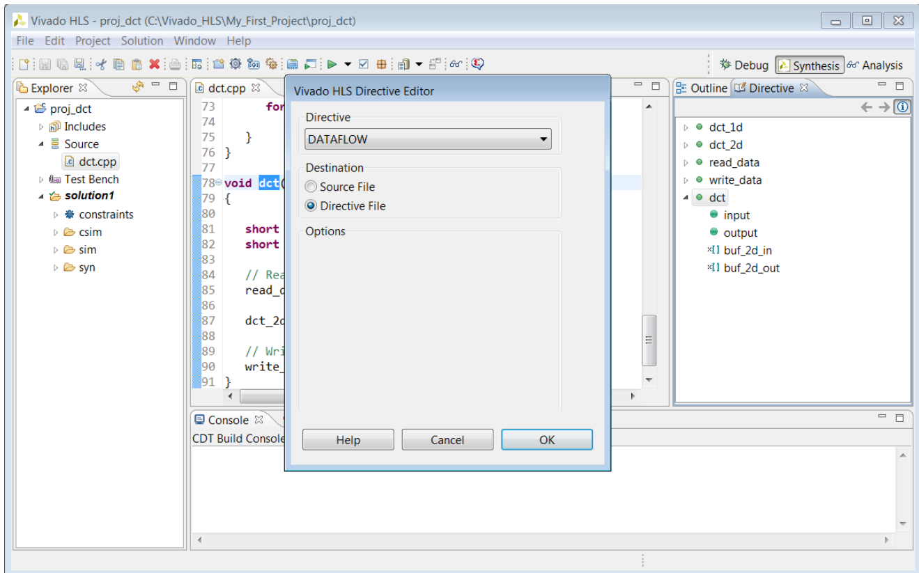
Figure 1-28: Adding Directives
