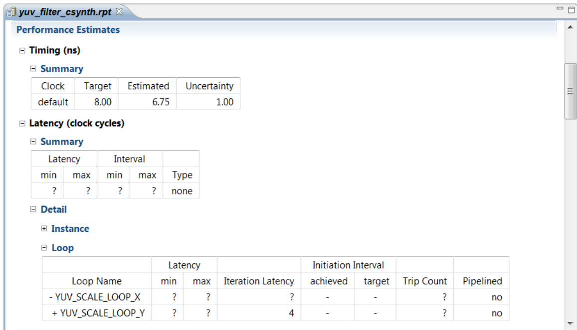
Figure 1-21: Analysis Perspective
