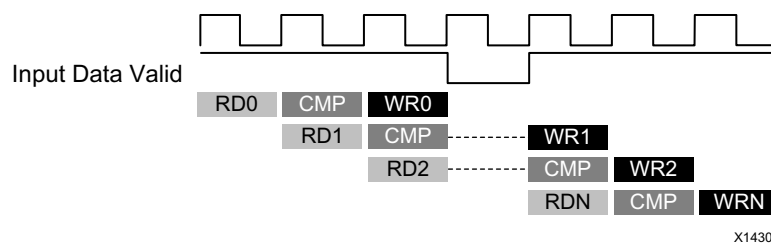
Figure 1-53: Loop Pipelining with Stall
