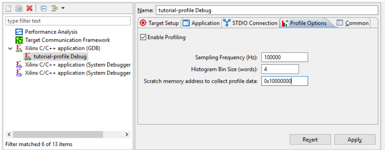
Figure 41: Profiling options.
