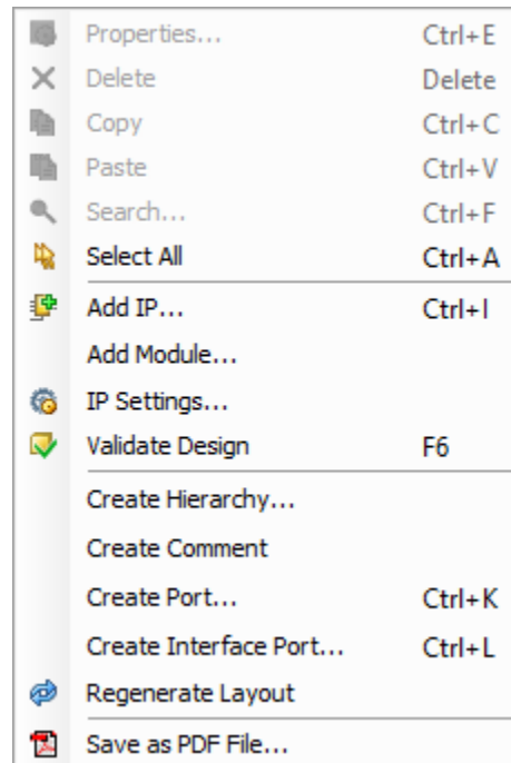
Figure 5: Add IP.
