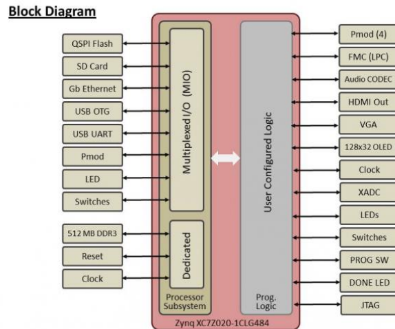
Figure 7: The Avnet ZedBoard BlockDiagram
